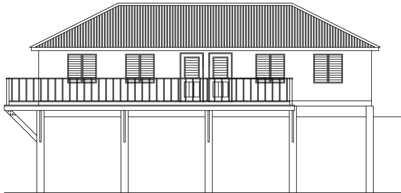
① REAR ELEVATION SCALE 1/8" = 1'-0"
