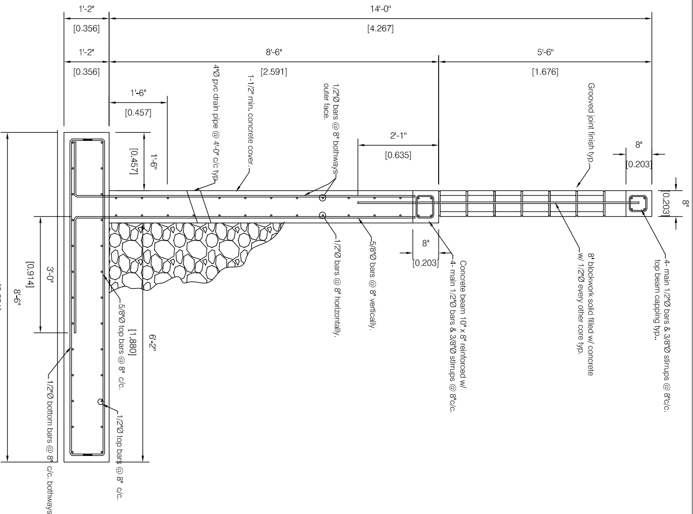
Retaining Wall Section (Virgin Islands) Scale nts
