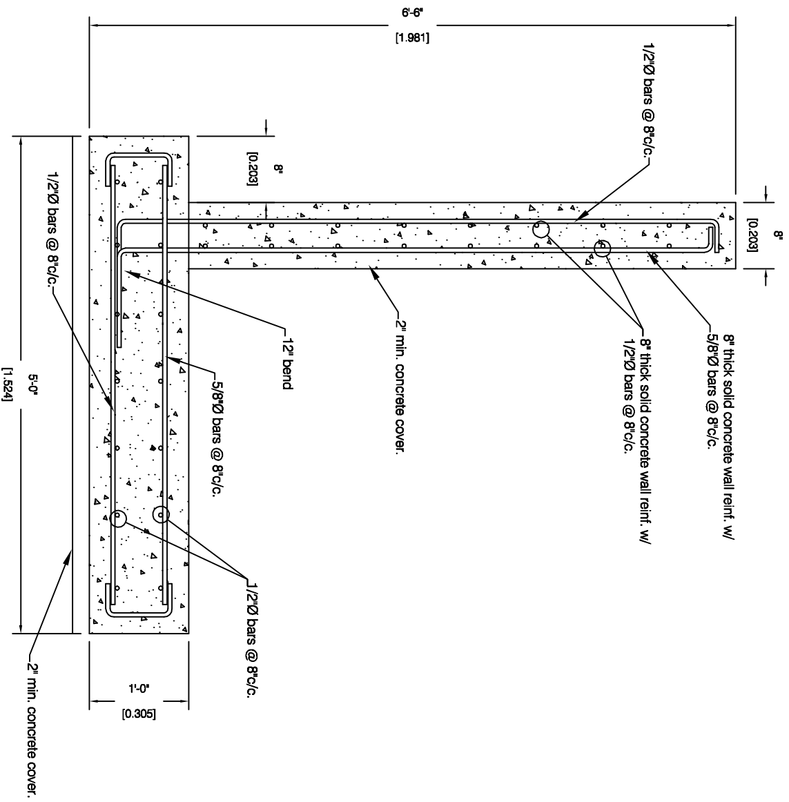
Proposed Retaining Wall (Salem) Scale 3/4" = 1'-0"
