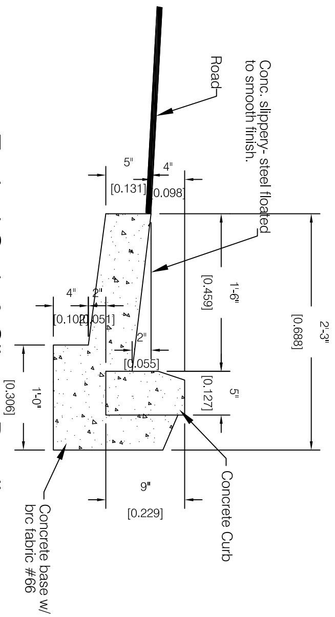
Typical Curb & Slipper Detail Scale NTS
